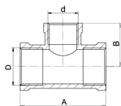
FT217 T - kus redukovaný MMM 3-way reduced brass fitting FFF
